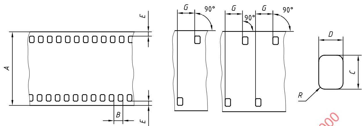
Figure 2 — Perforations for 135-size film (see Table 2)
