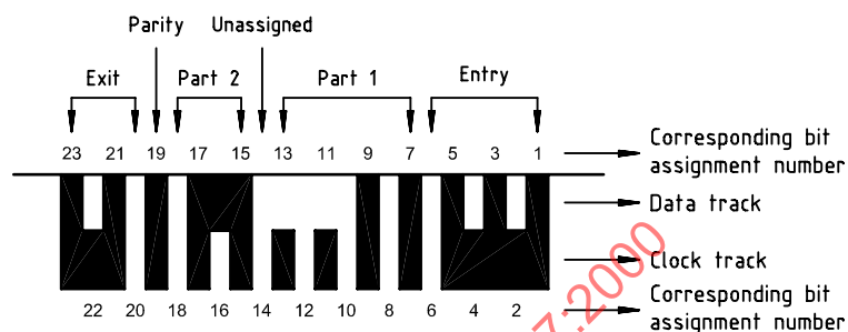
e) Latent-image dual-track bar-code
