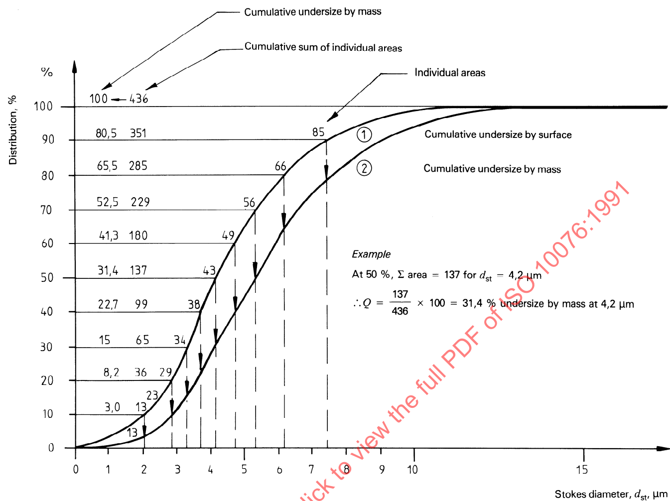
Figure A.1 — Graphical transformation of undersize by surface to undersize by mass
