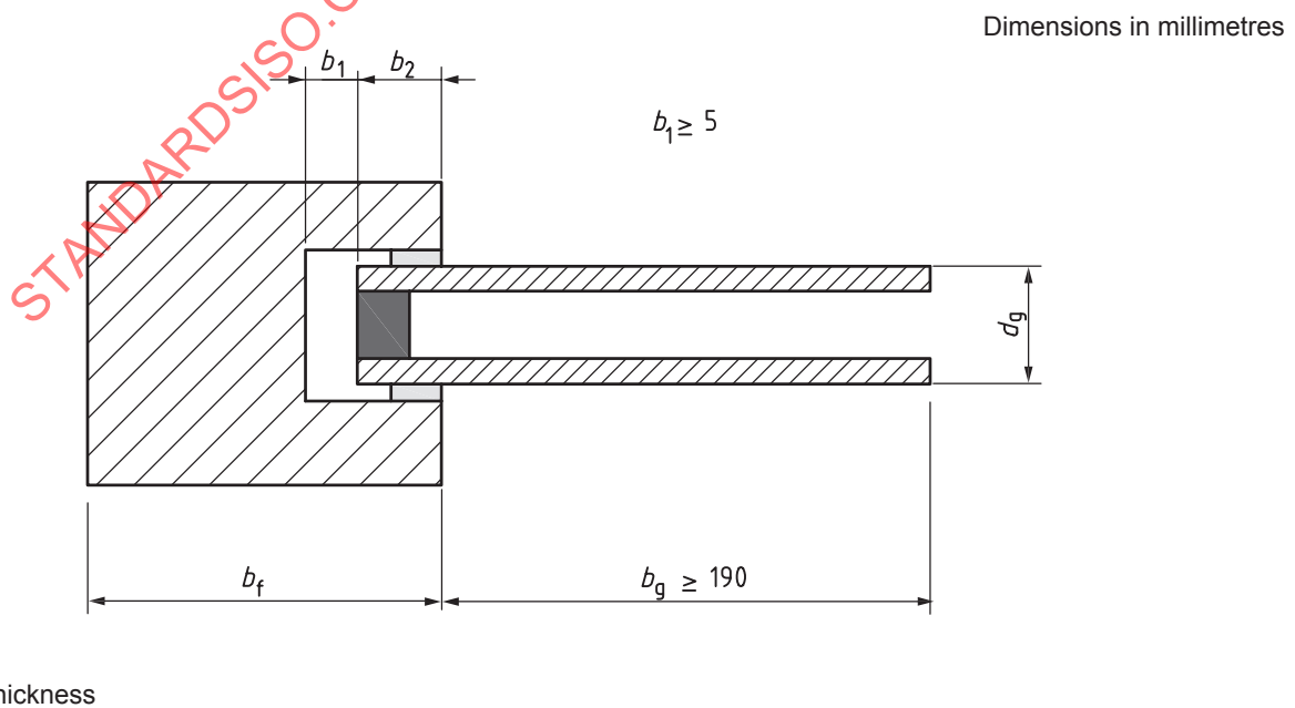
Figure C.2 — Schematic of profile section with glazing installed
