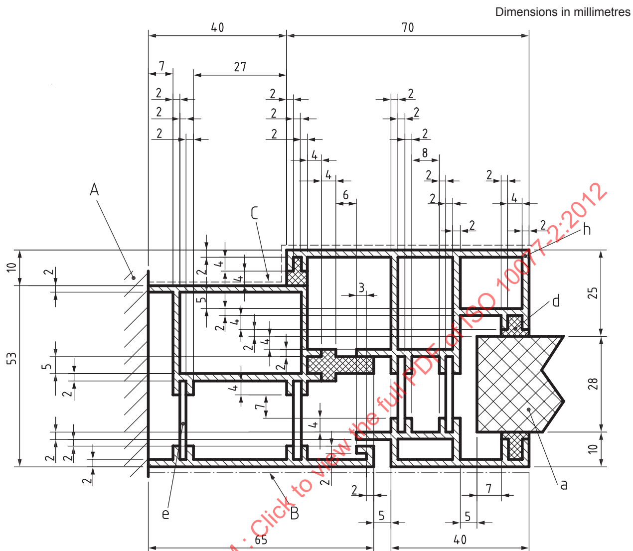
Figure D.1 — Aluminium frame section with thermal break and insulation panel ( b_f = 110 mm)
