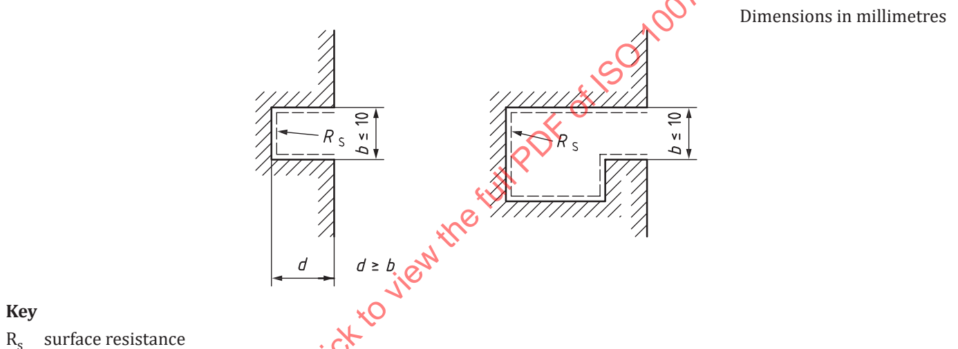
Figure 10 — Examples for slightly ventilated cavities and grooves with small cross section
