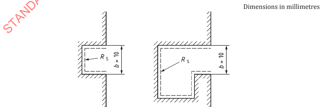
Figure 11 — Examples for well-ventilated cavities and grooves
