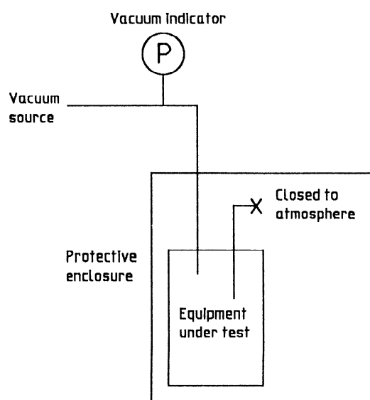
Figure A.2 — Apparatus for testing resistance to implosion, cracking or permanent deformation
