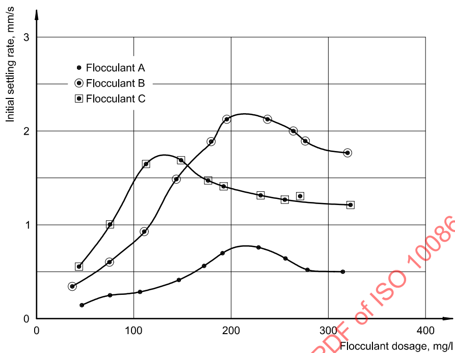
Figure A.2 — Plots of free-settling rate as a function of flocculant dosage for different flocculants
