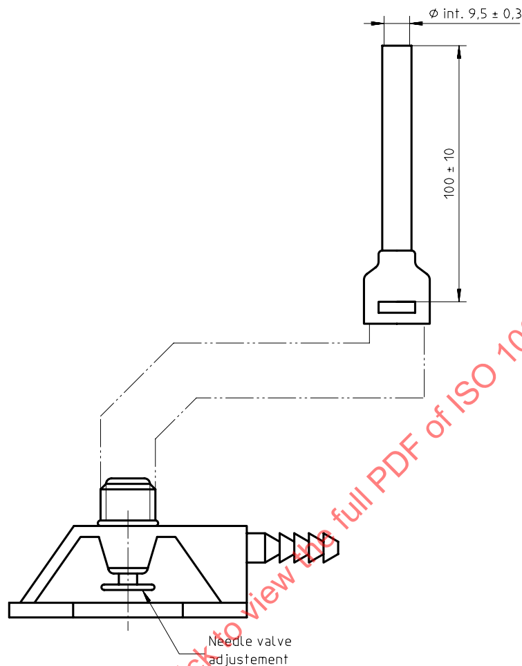
Figure 7 — Ignition source P/PF2
