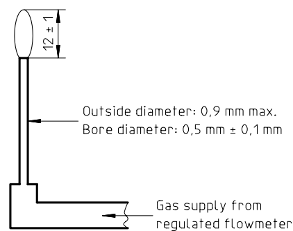
Figure 3 — Ignition source P/DF1
