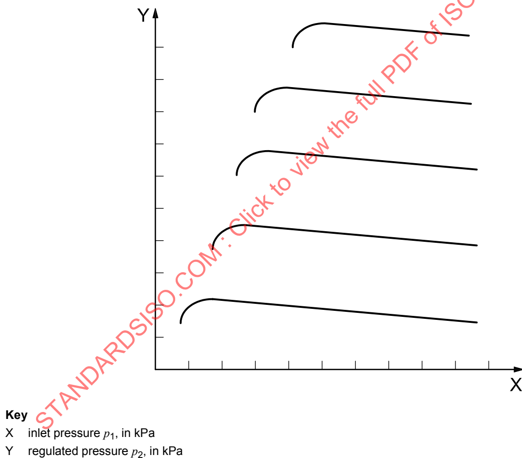
Figure 4 — Pressure regulation characteristic curves
