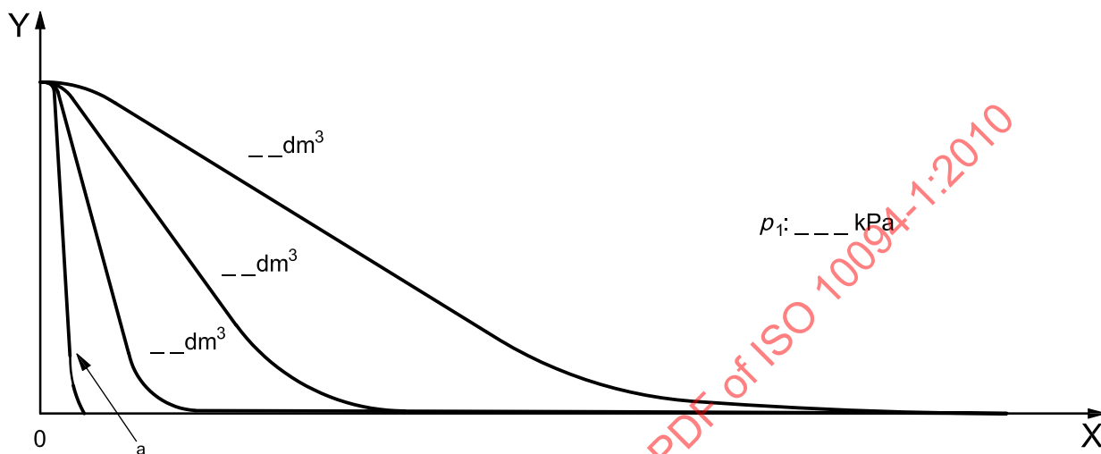
a) Case of pressure responses without oscillations
