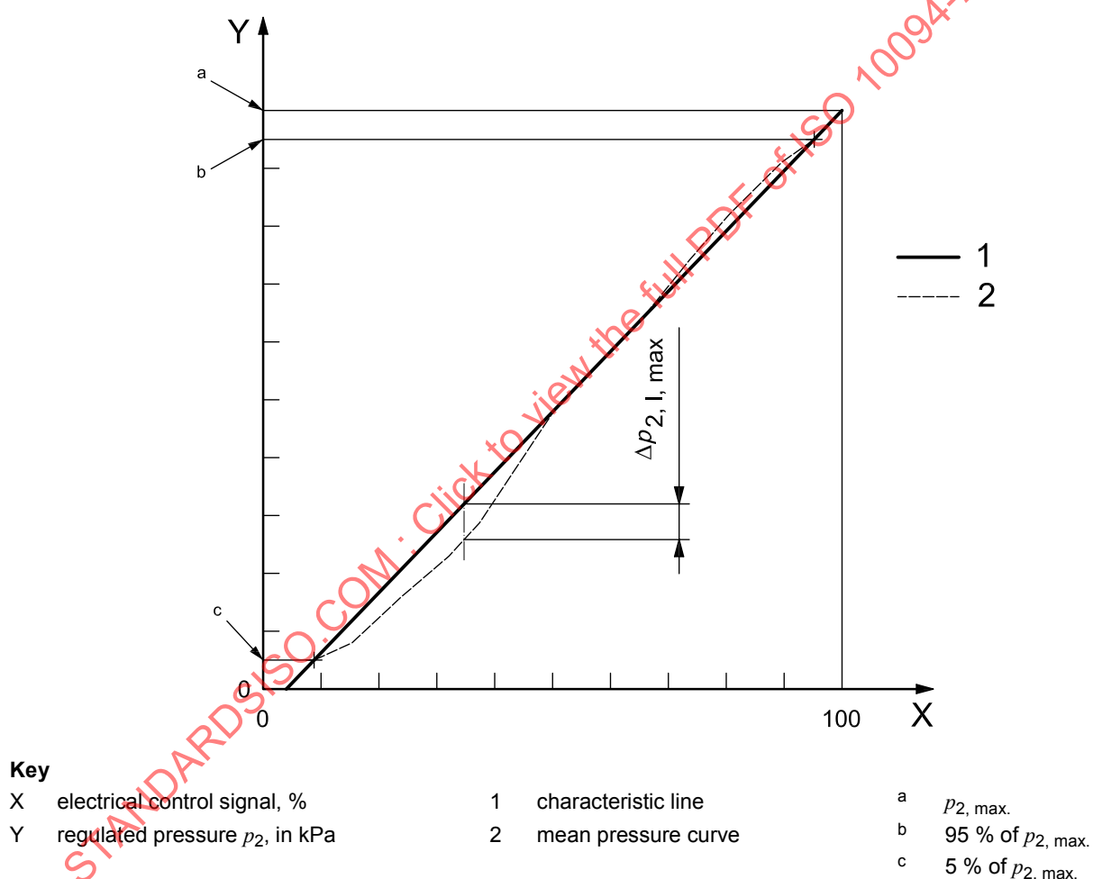
Figure 3 — Representation of the maximal scattering of linearity
