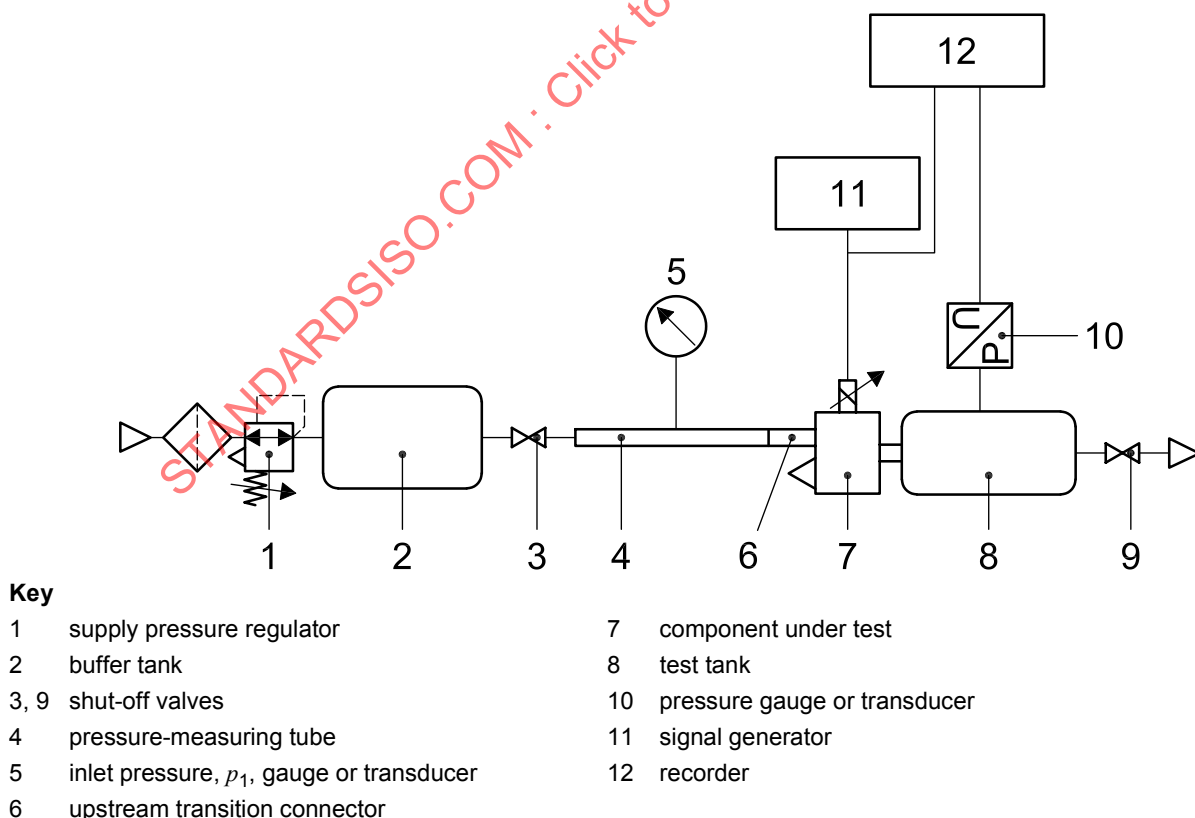
Figure 9 — Test circuit for dynamic characterization with a tank
