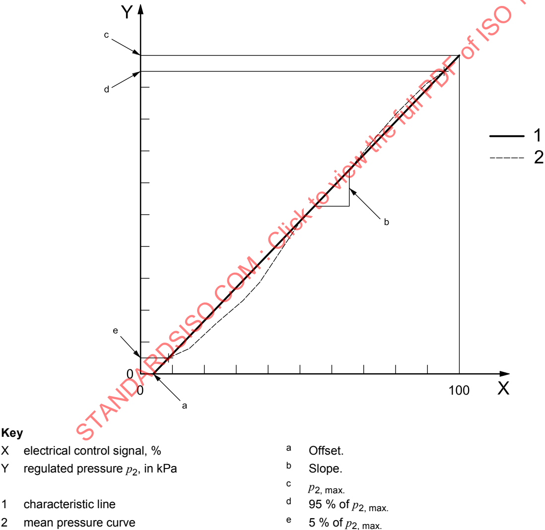
Figure 2 — Determination of the characteristic curve
