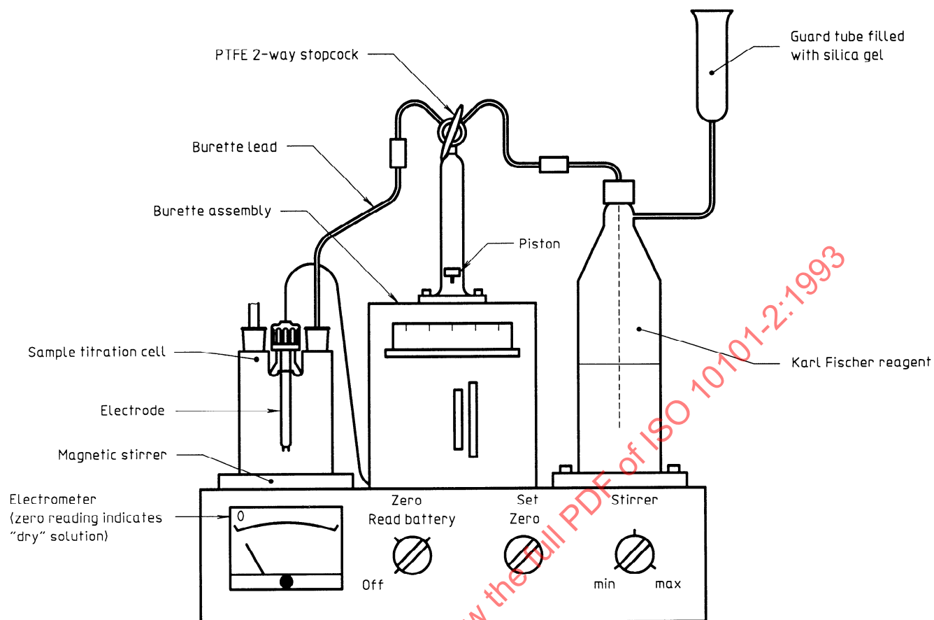
Figure A.2 — Titration apparatus — Typical assembly
