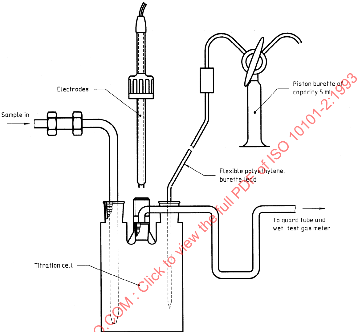
Figure A.1 — Detail of titration cell
