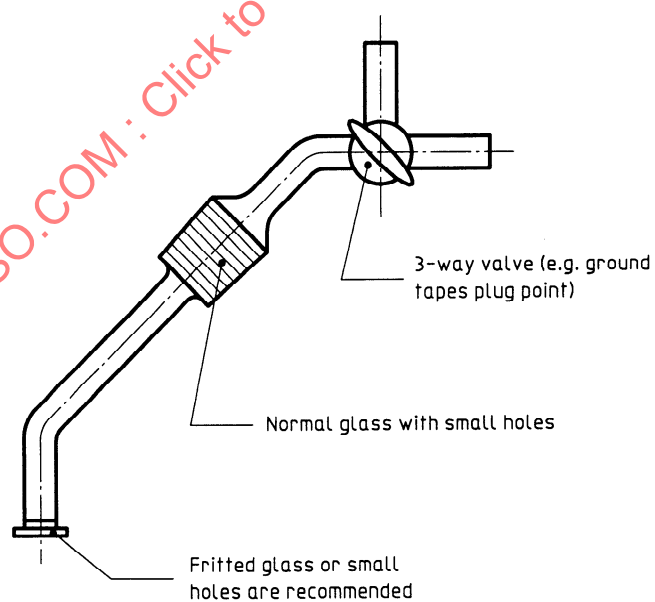
Figure 3 — Gas inlet with 3-way valve
