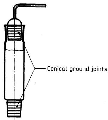
Figure 4 — Drying tube in the gas outlet line
