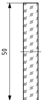
Figure 3 — Rectangular cylindrical lens element
