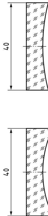
Figure 6 — Square toric lens element
