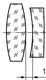
Figure 36 — Air space between lens elements
