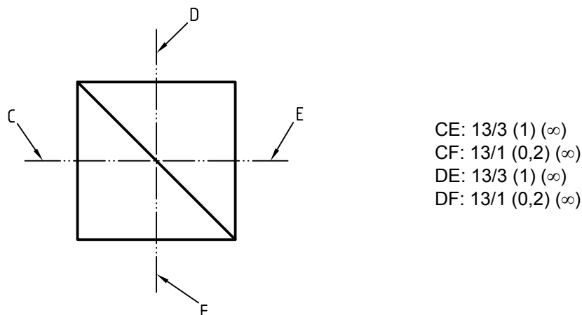
Figure 4 — Indication of the wavefront quality specification for an element having multiple test paths
