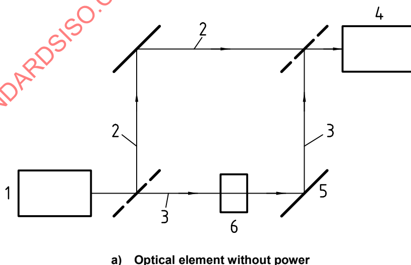
Figure B.1 — Testing an optical element in single-pass
