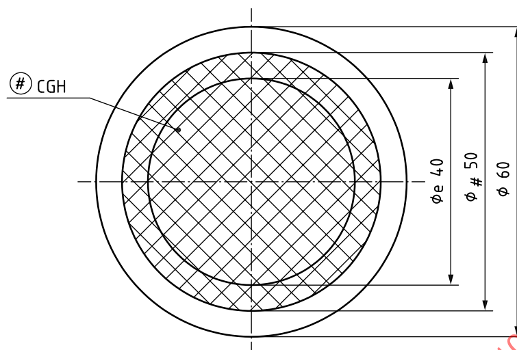
Figure 6 — Indication of the diffractive region and corresponding diffractive test region
