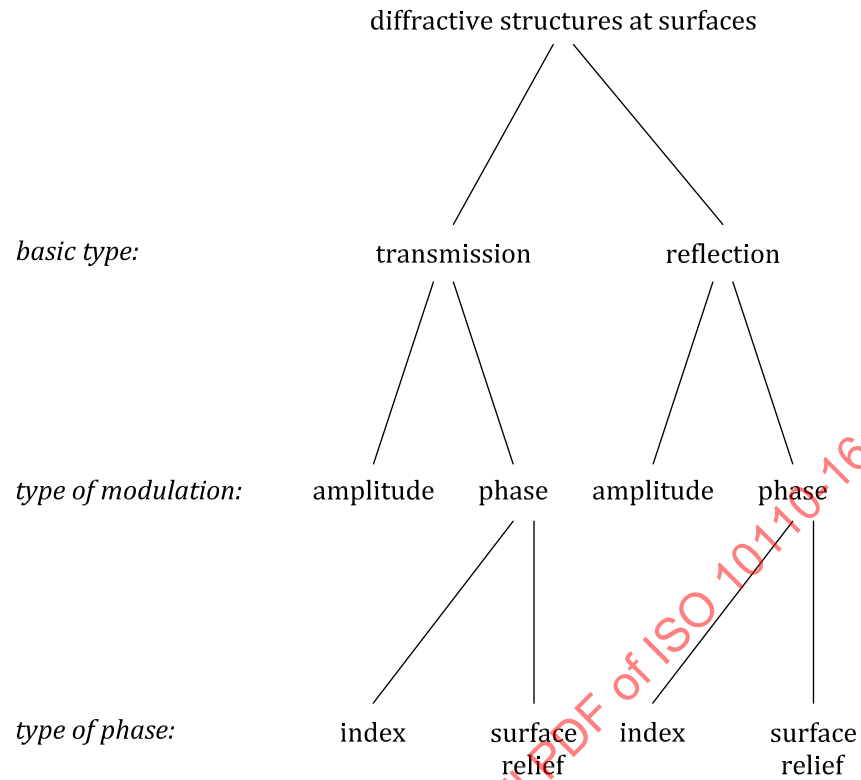
Figure A.2 — Classification scheme of diffractive structures
