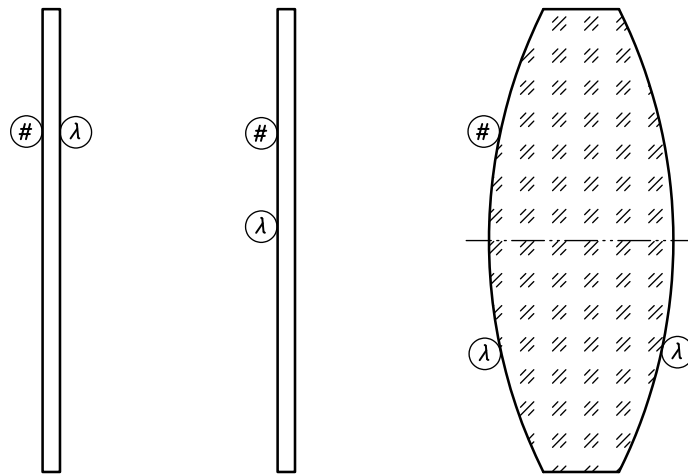
Figure 3 — Usual marking of a diffractive surface in side view or sectional view with symbols on the outside
