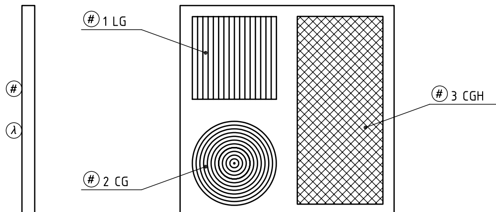
Figure 5 — Hatching, numbering and classification of several diffractive structures on drawings
