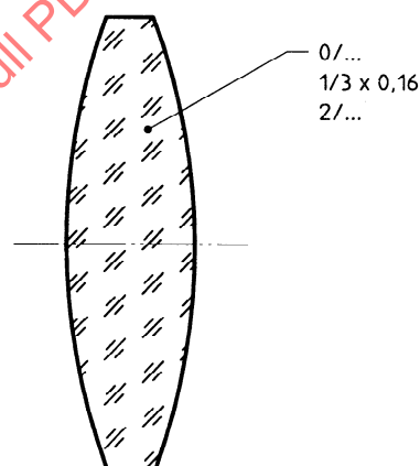
Figure 1 — Example of tolerance indication for bubbles and other inclusions
