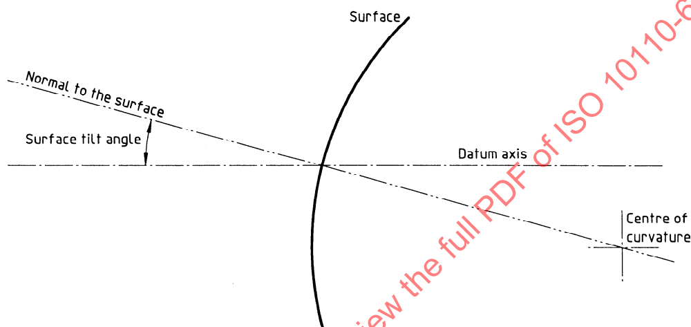
Figure 1 — Tilt angle of a single spherical surface
