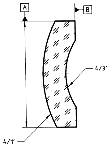
Figure 6 — Datum axis referencing a plane and the central point of an optically effective surface
