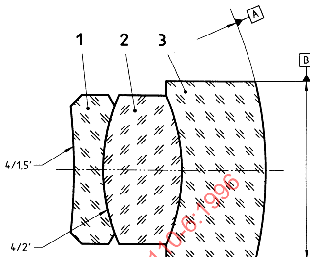
Figure 12 — Datum axis referencing centre of curvature and central point of the same surface
