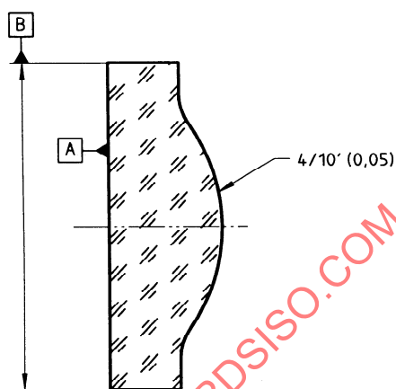
Figure 7 — Centring tolerance for an aspheric surface
