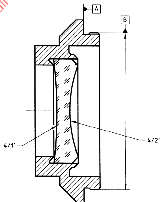
Figure 13 — Datum axis referencing mechanical elements
