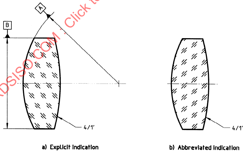
Figure 5 — Datum axis referencing centre of curvature and central point of the same surface
