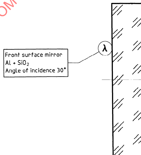
Figure 3 — Example of functional coating indication with specification of material
