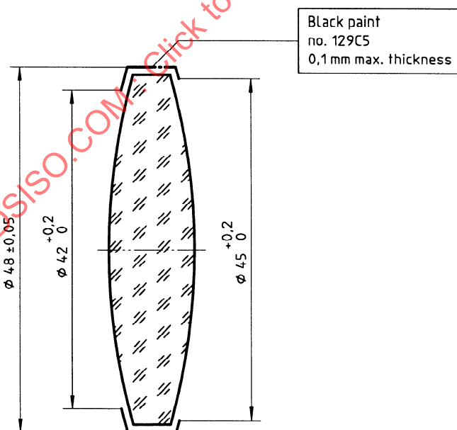
Figure 5 — Example of protective surface treatment indication (The outer diameter of 48 \pm 0.05 refers to the part after painting)
