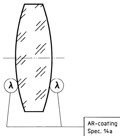
Figure 1 — Example of functional coating indication referencing separate specification
