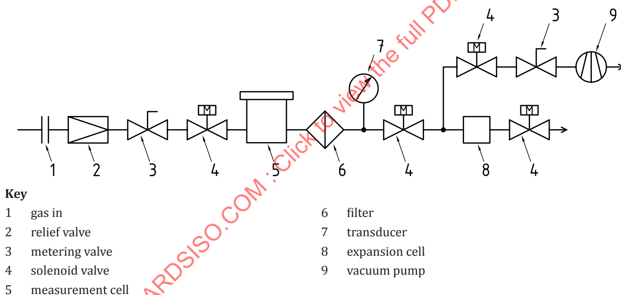
Figure 3 — Schematic examples of a gas pycnometer
