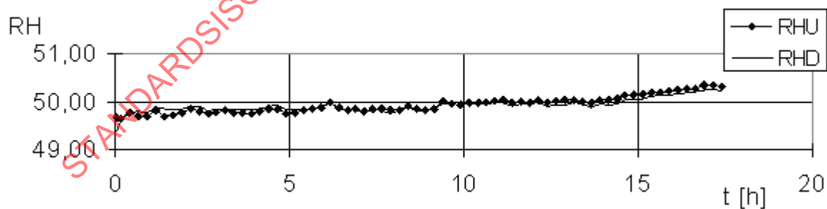
b) Example verification of relative humidity accuracy and oscillation
