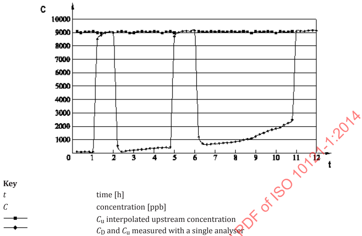
Figure 3 — Example of a concentration graph when using a single analyser for C_U and C_D
