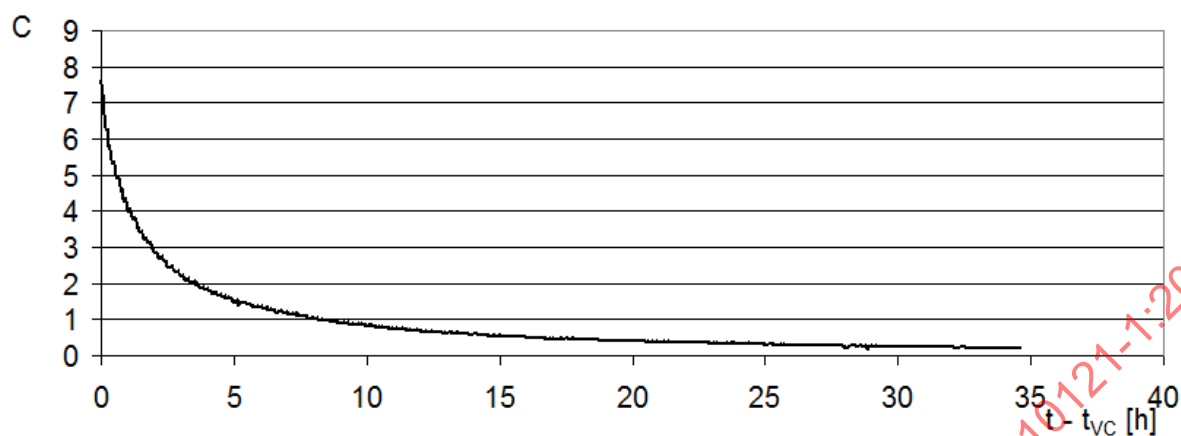
Figure 6 — Example of retentivity test, C vs. t, (see 6.4)
