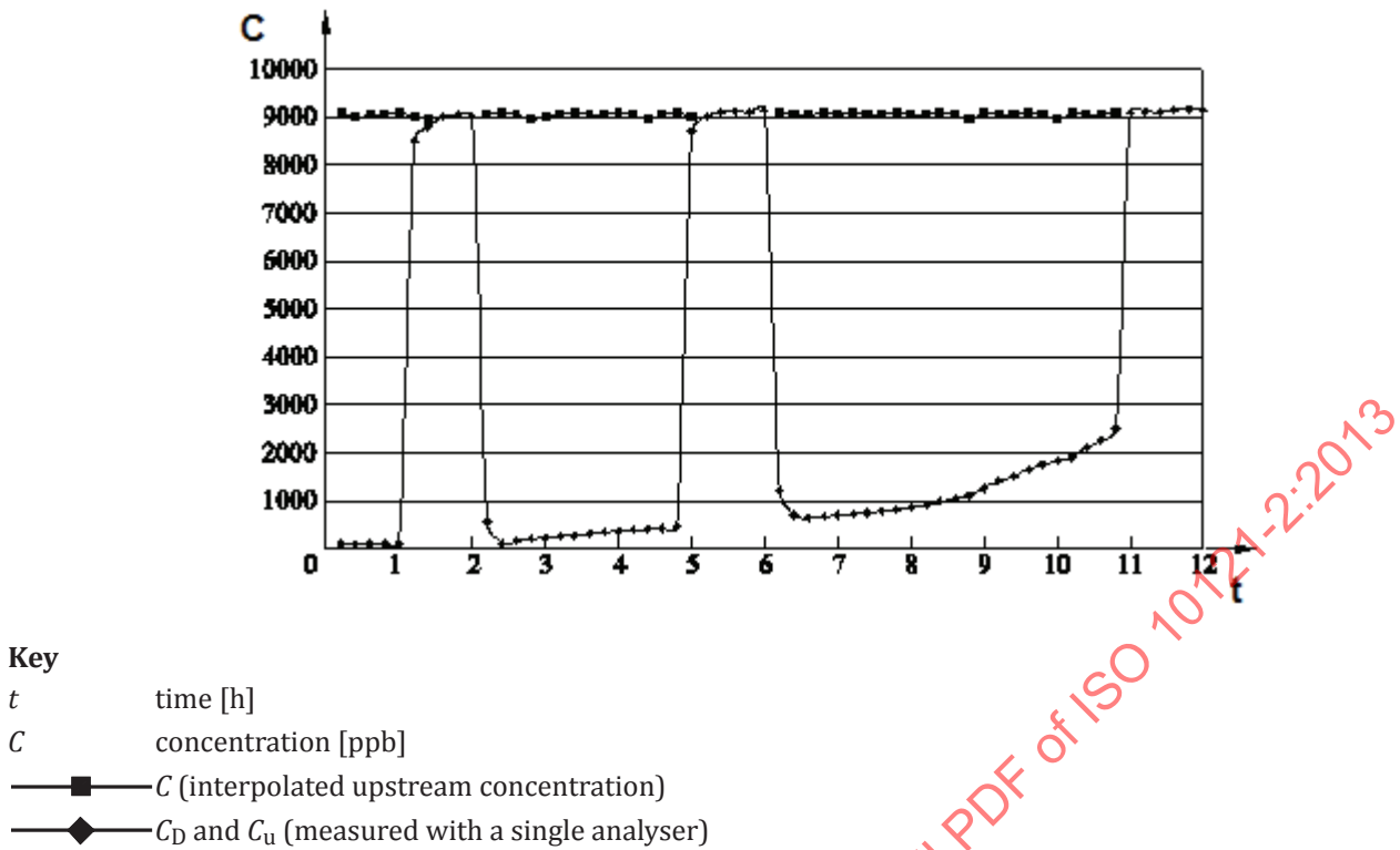
Figure 4 — Example of a concentration graph when using a single analyser for C_U and C_D
