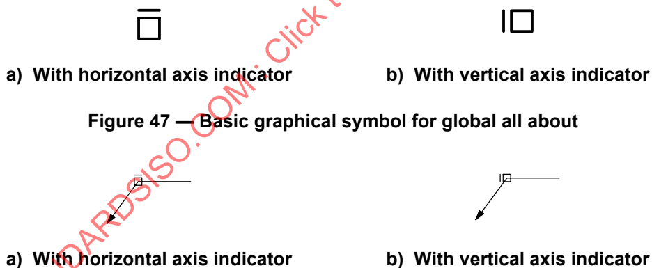
Figure 48 — Graphical symbol for indication of global all about condition used on leader and reference lines
