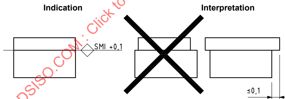
Figure 20 — Permissible surface mismatch (SMI) between two mating mould components when specified with \pm sign on the upper mould component
