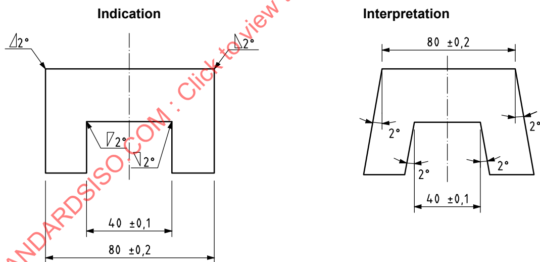
Figure 64 — Draft resulting from use of single inclination symbols (2nd example)
