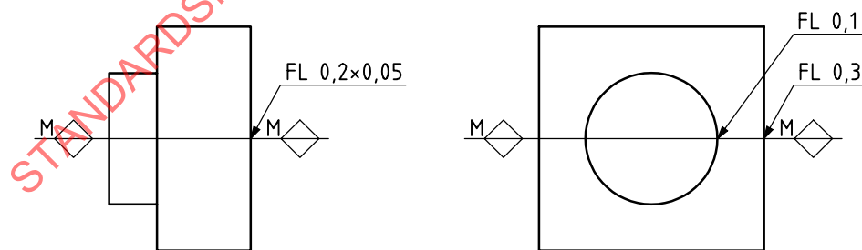
Figure 33 — Example of indication of flash at individual features
