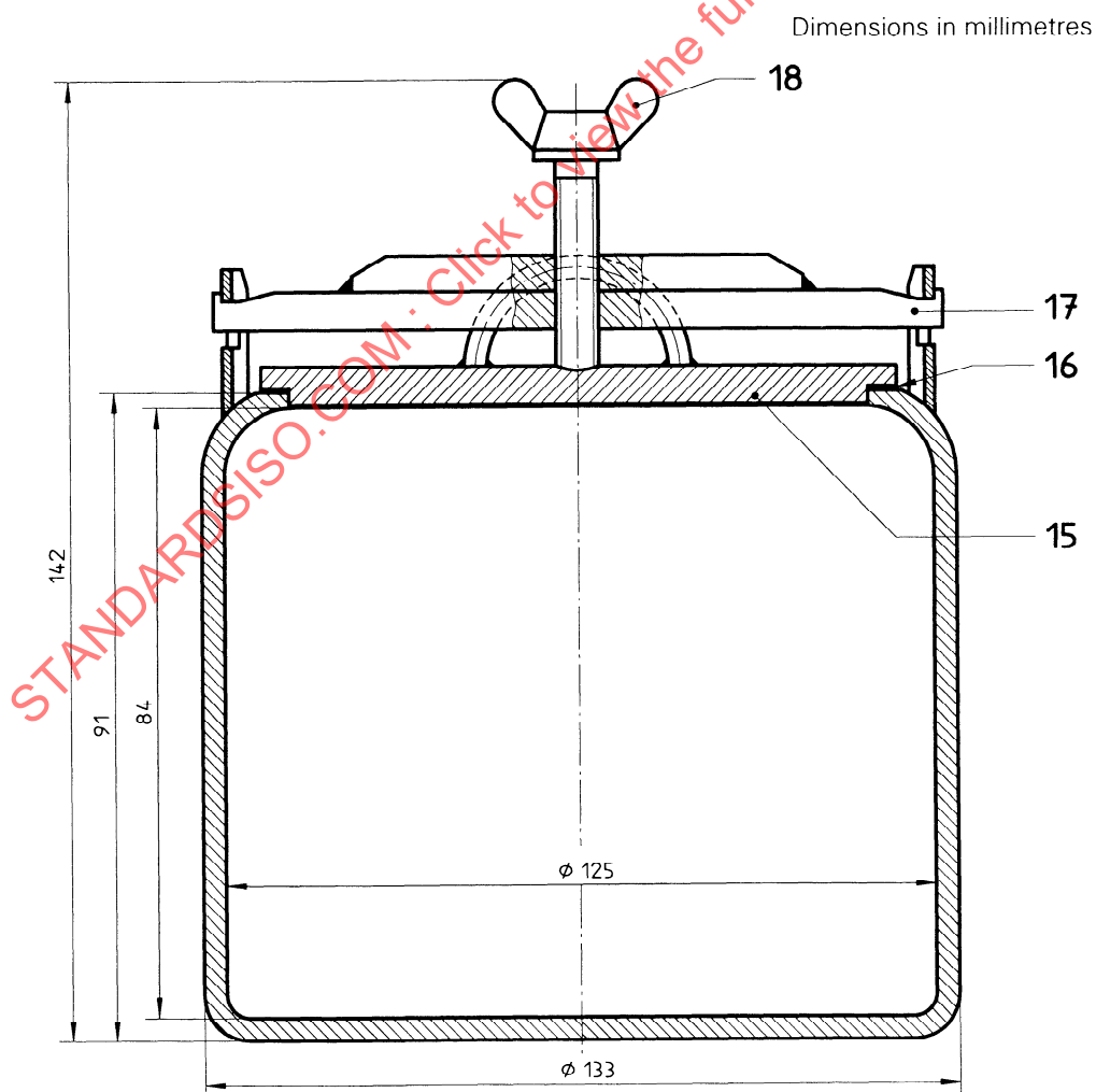
Figure 5 — Grinding vessel
