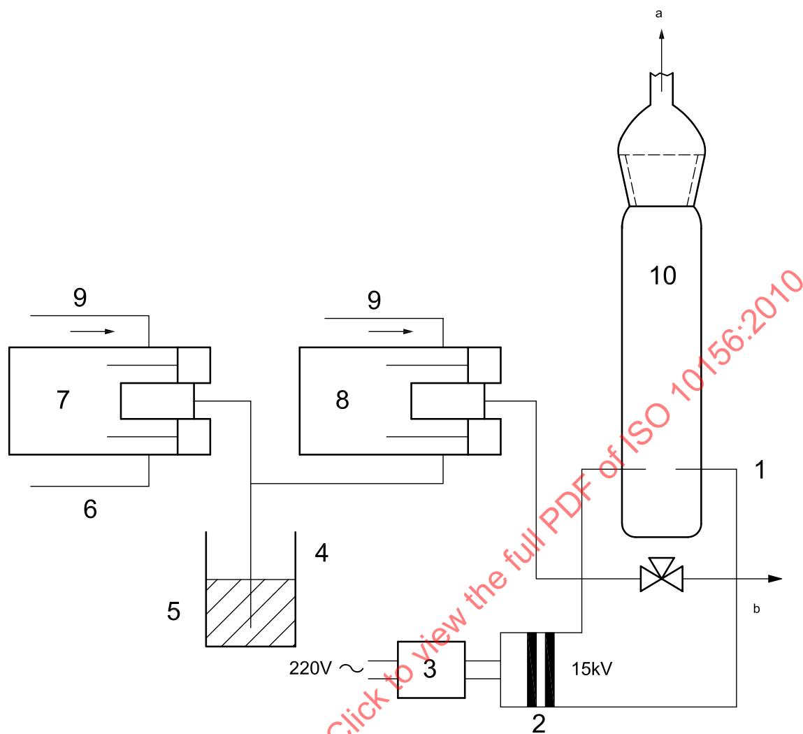
b) Apparatus suitable for testing a mixture of gases
