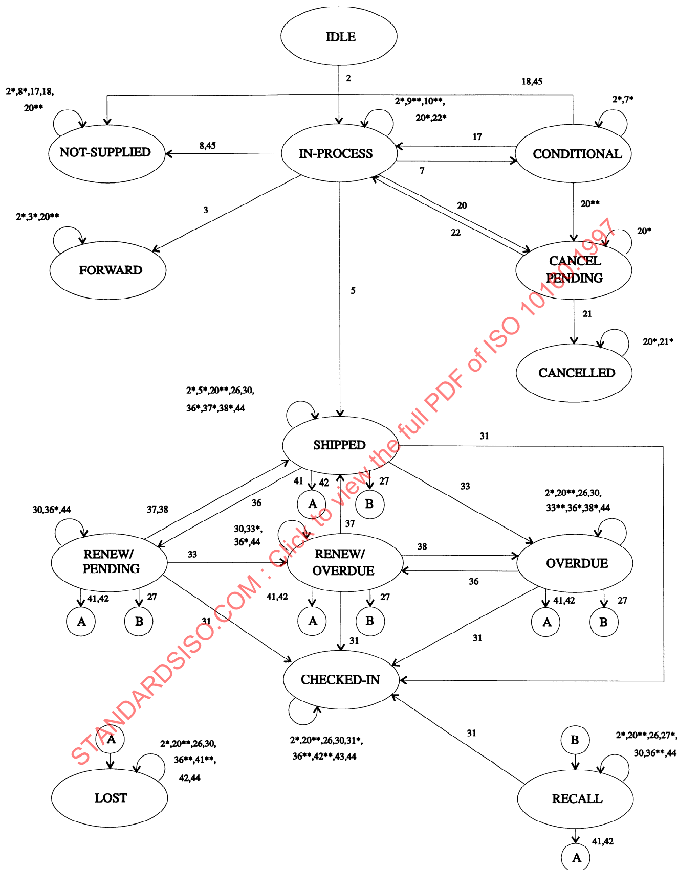
Figure 10 State Transitions for Responder: Returnable Item (In-Sequence Messages Only)
