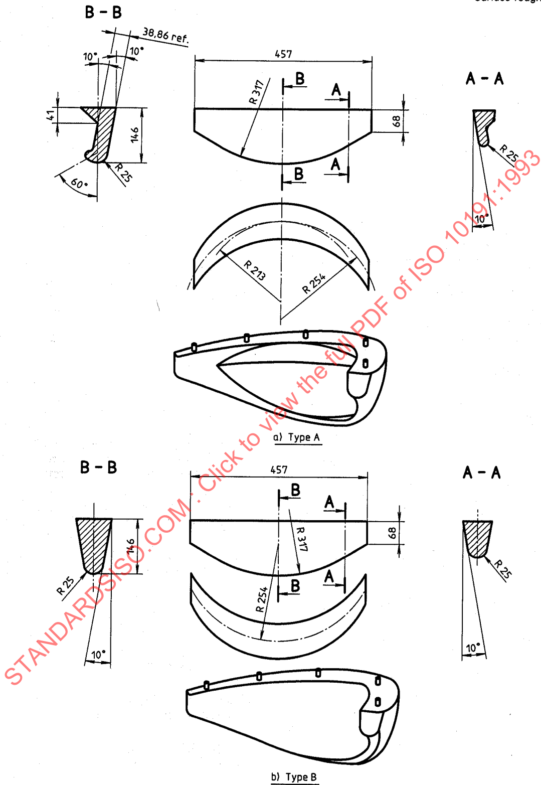
Figure 1 — Diagrams of bead unseating blocks
