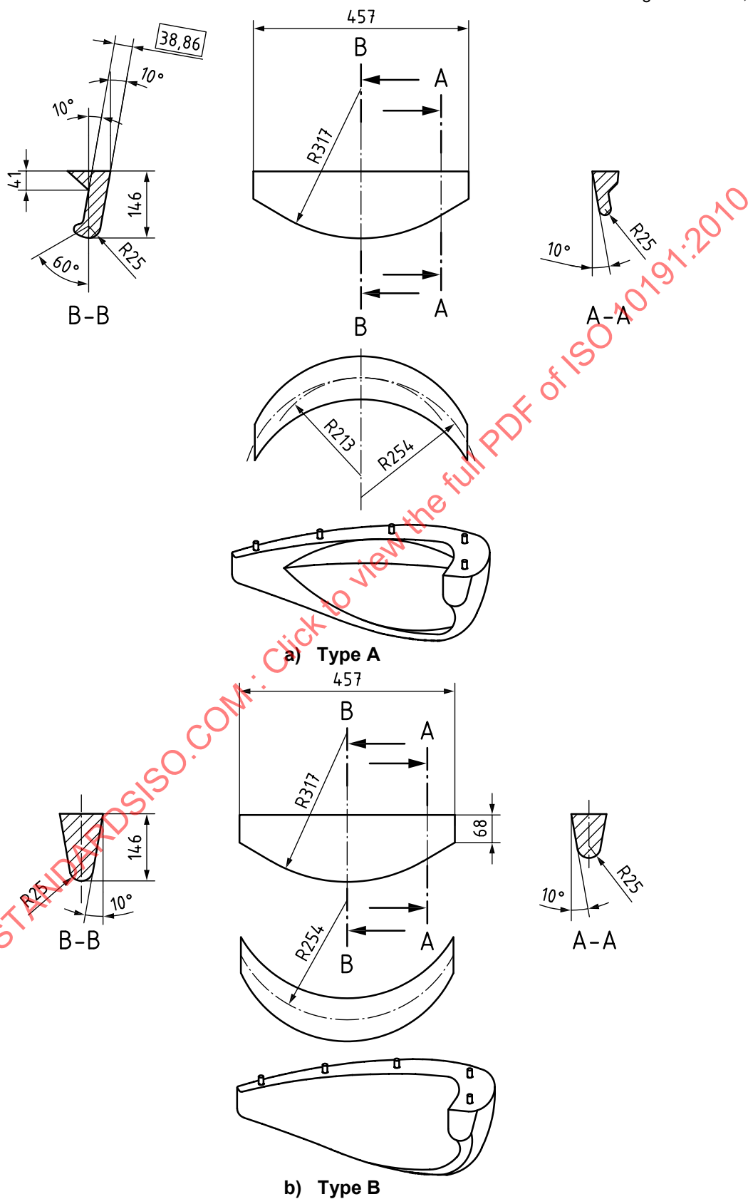
Figure 1 — Diagrams of bead unseating blocks
