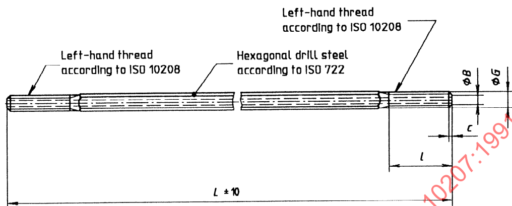
a) Normal equipment
