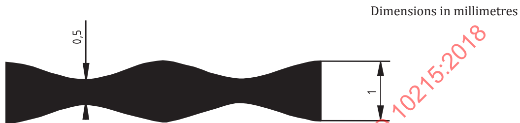
Figure 4 — Example of distortion of image — Line of Grade 5
