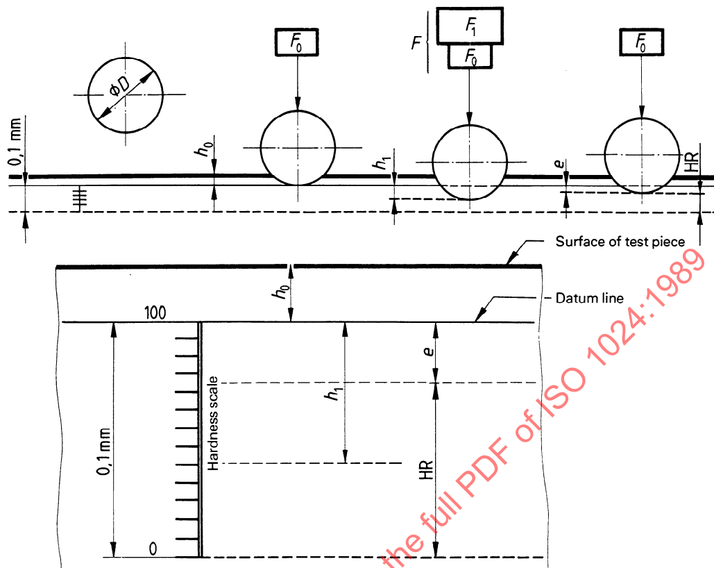
Figure 2 — Test with steel ball
