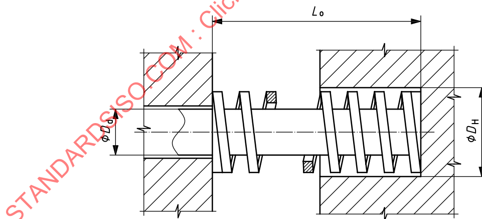
Figure 1 — Compression springs
