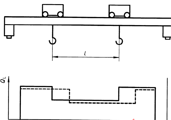
a) A minimum distance l between two crabs is required in order to use the full rated capacity of the crabs. With a shorter distance the rated capacity is reduced (mainly in order to reduce bridge weight and keep wheel loads within allowable limits).
