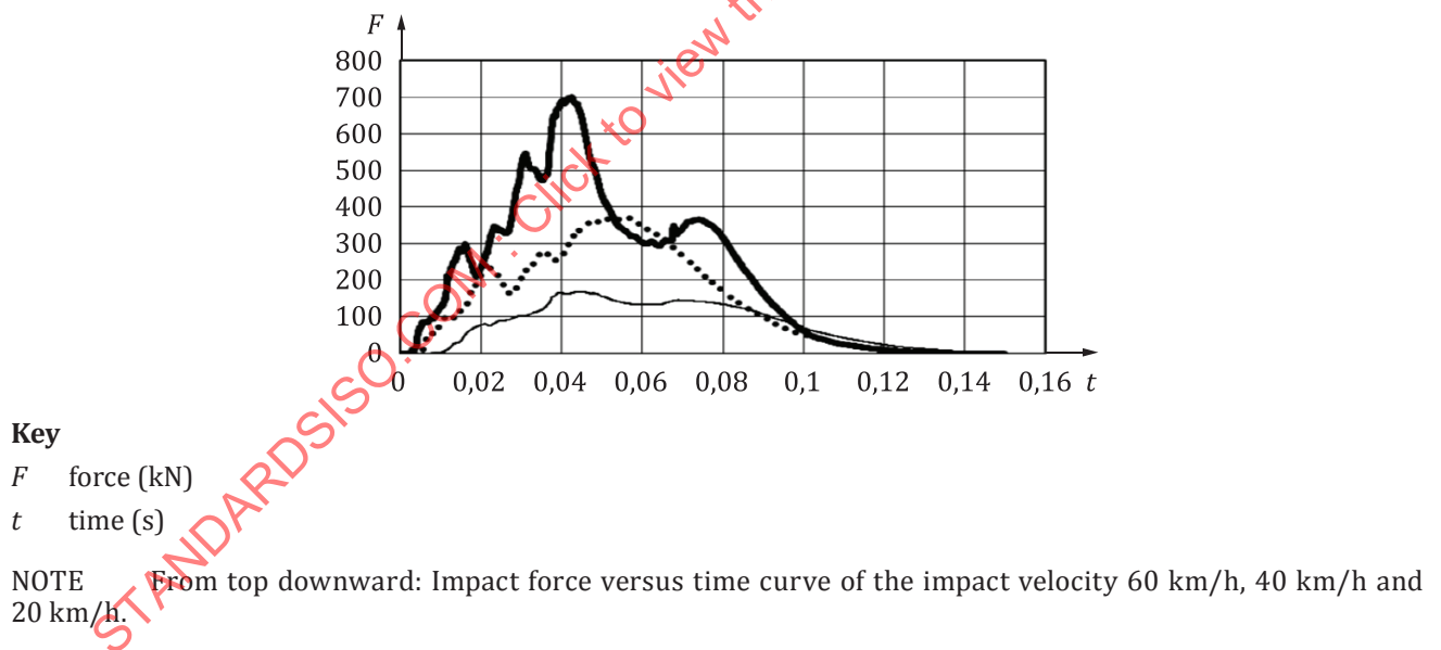
Figure A.12 — Impact force versus time curve for each impact velocity
