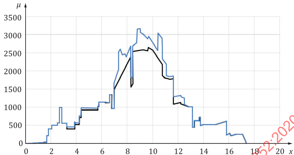
Figure A.22 — Example of mass per unit length, \mu(x) , for the F-4 Aircraft with (upper curve) and without (lower curve) skids and rockets [19]
