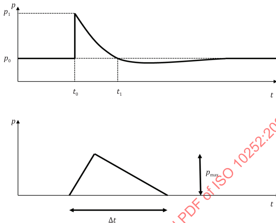
Figure B.11 — Realistic pressure wave and triangular simplification (relative to the atmospheric pressure)
