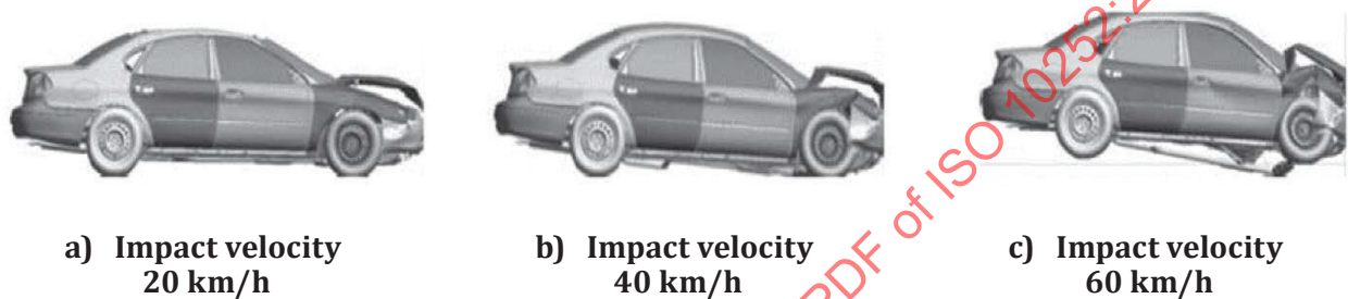
Figure A.11 — Maximum deformations for each impact velocity
