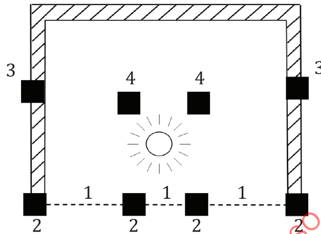
Figure B.1 — Floor plan with differently situated columns
