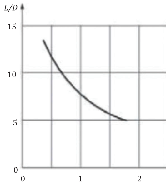
Figure B.9 — L/D values for dust with a K_{St} value of less than 30 000 kN/ms and an initial flow velocity of between 2 m/s and 20 m/s, for design overpressure <20 kN/m 2
