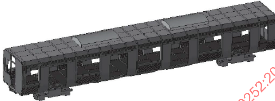
Figure A.15 — Finite element model of the train [11]
