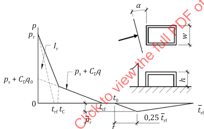
Figure B.12 — Front wall loading, normal reflection
