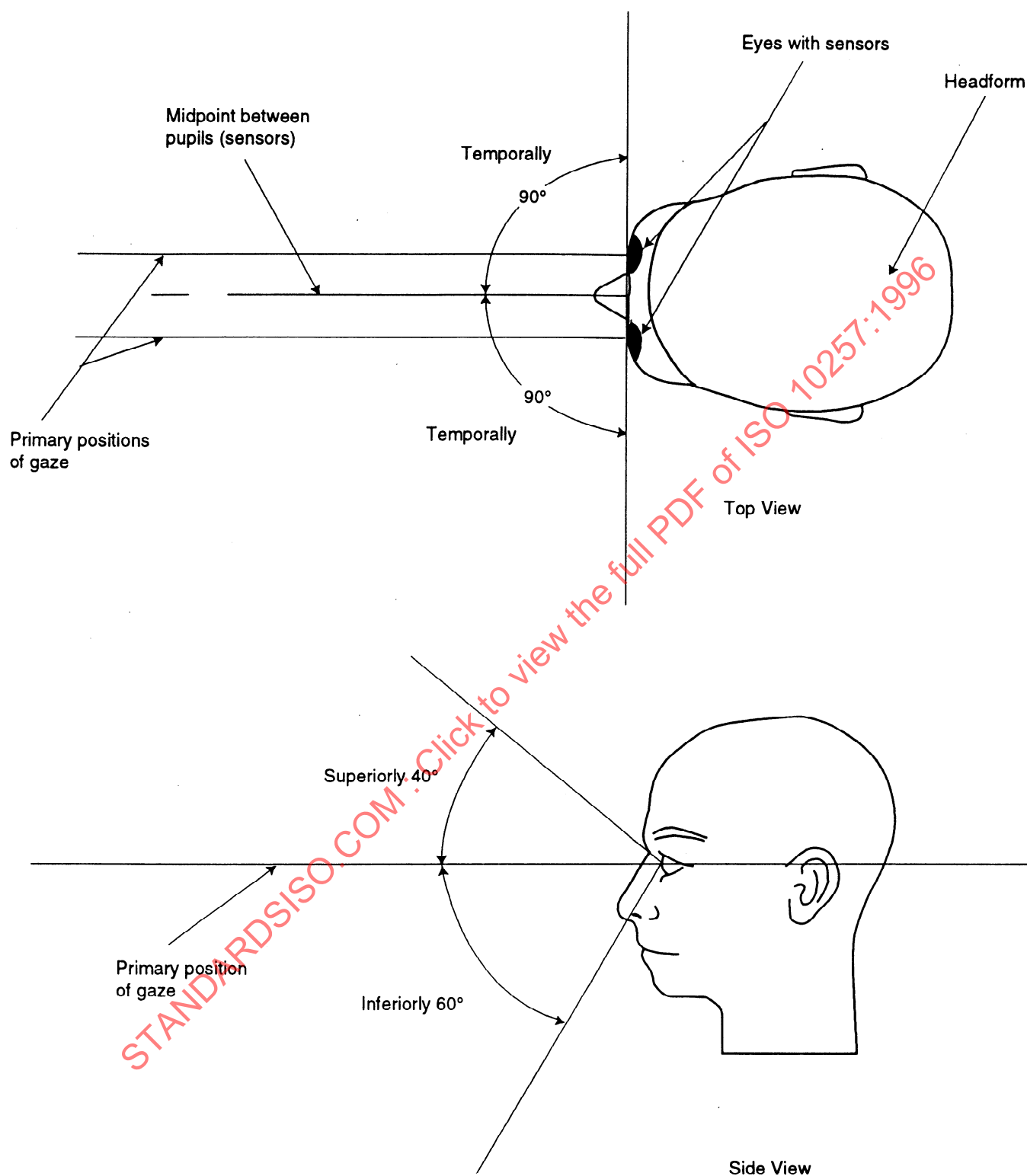
Figure 5 — Peripheral Field of Vision Testing (for Types 1A, 1B, 1C, 2, and 3)
