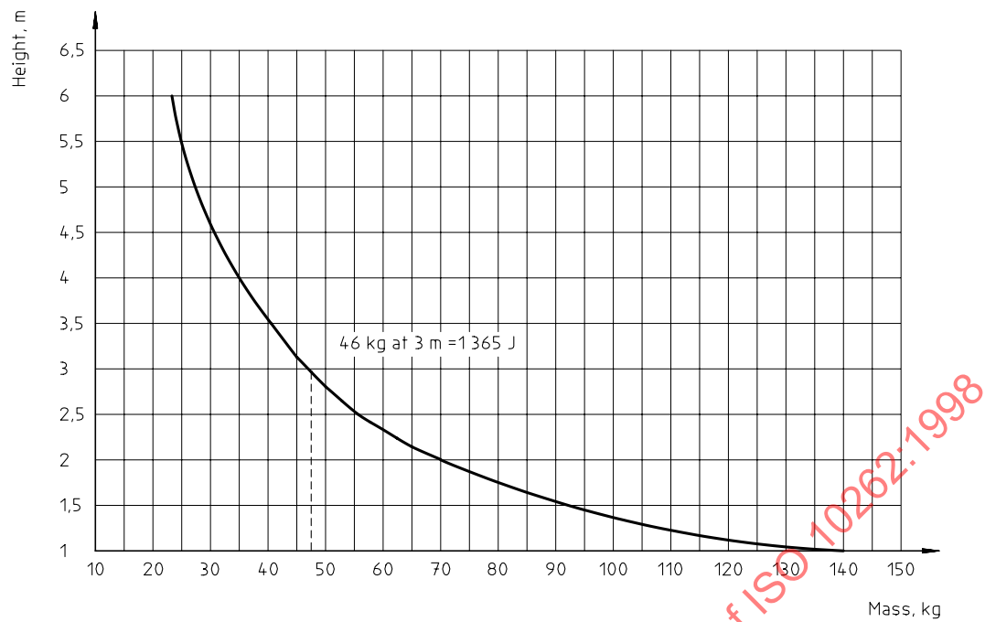
a) Level I energy requirement curve Energy required: 1 365 J
