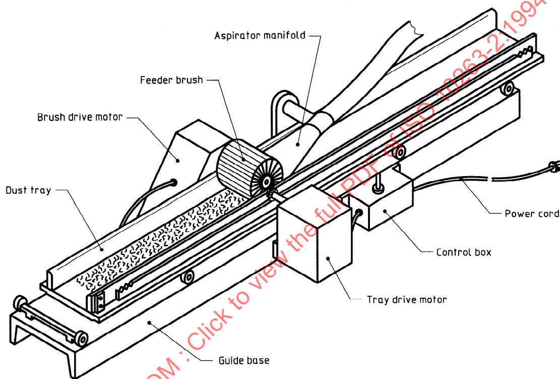
Figure 2 — Dust feeder
