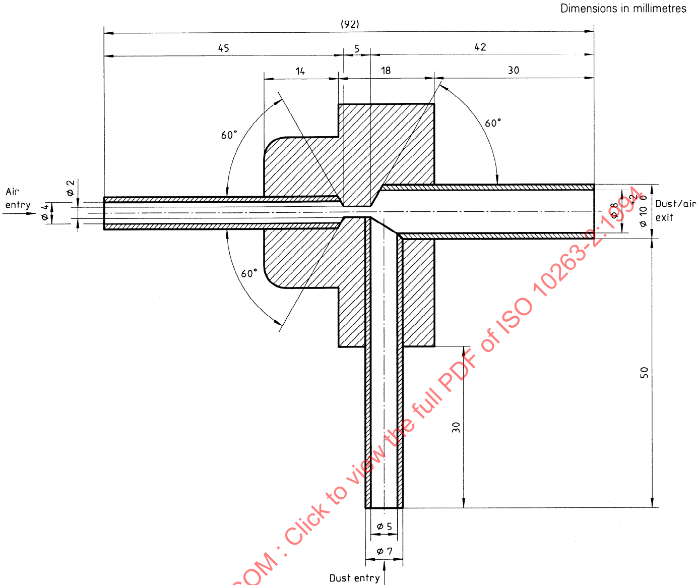
Figure 3 — Dust injector
