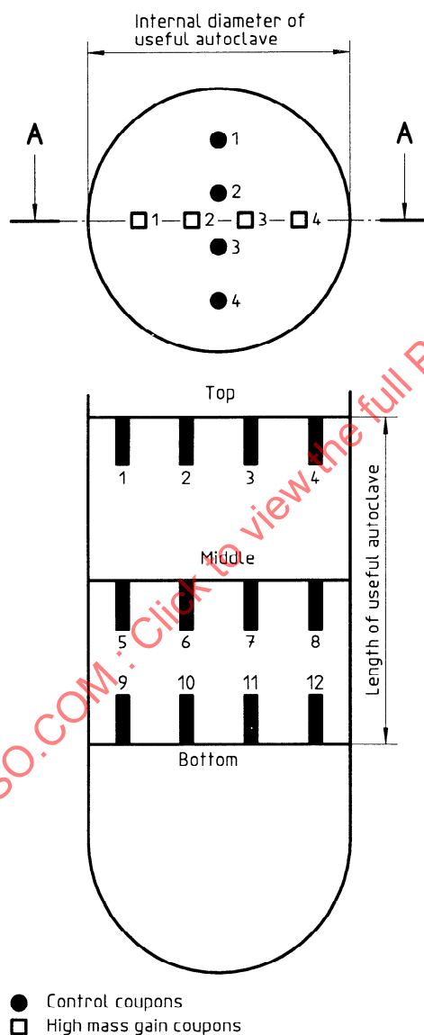
Figure 1 — Control coupon and high mass gain coupon positioning for establishing mass gain mean and standard deviation
