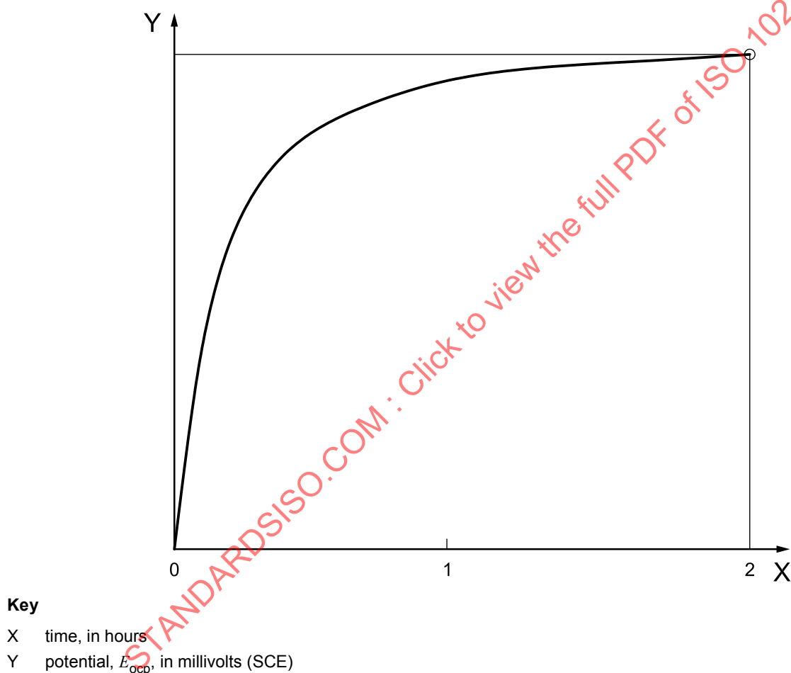
Figure 3 — Open-circuit potential versus time
