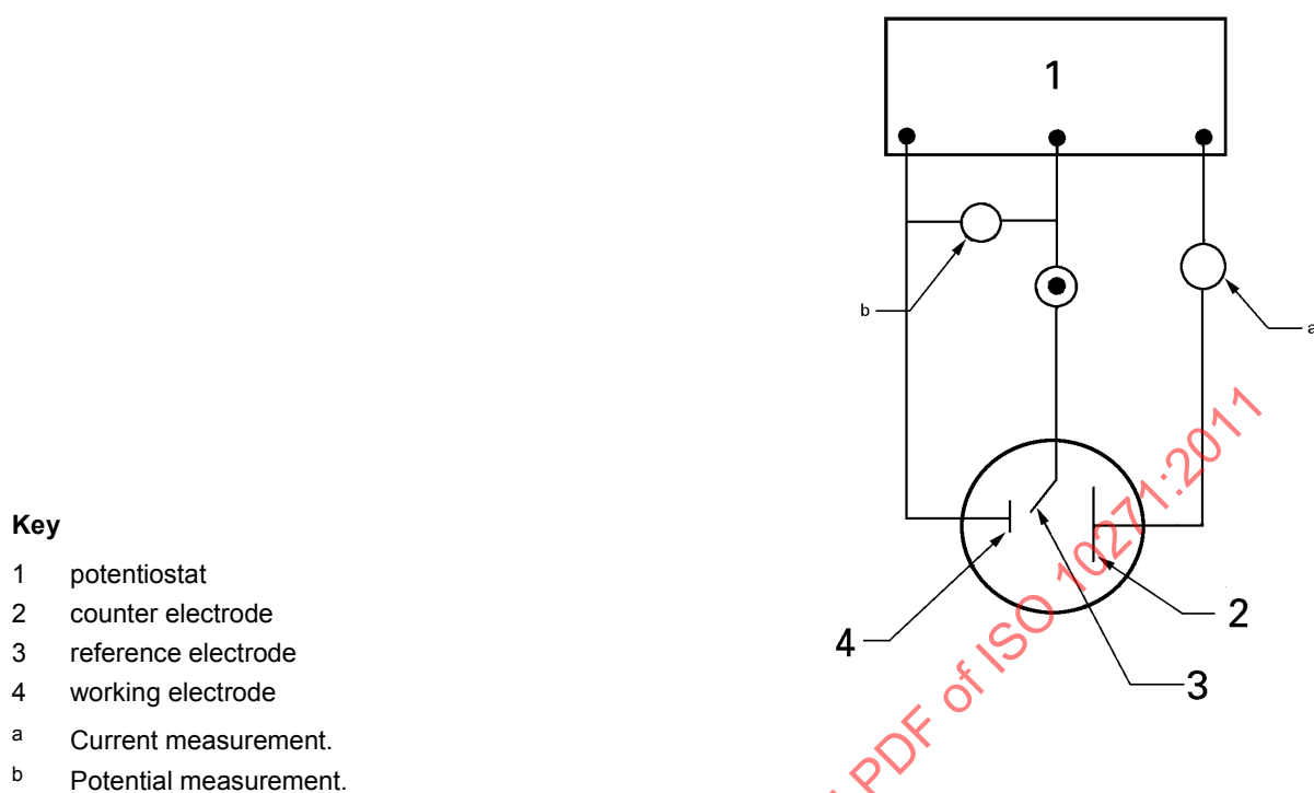
Figure 1 — Schematic diagram of measuring circuit
