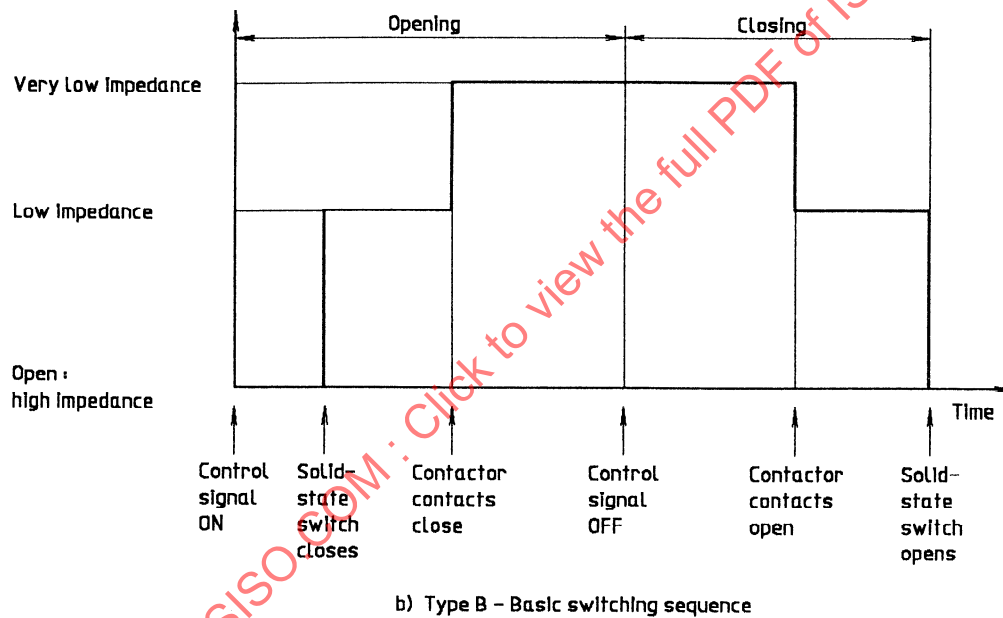
Figure 3 — Timing sequence diagram
