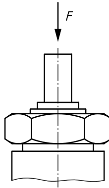
Figure 14 — Application direction for the valve spindle impact test
