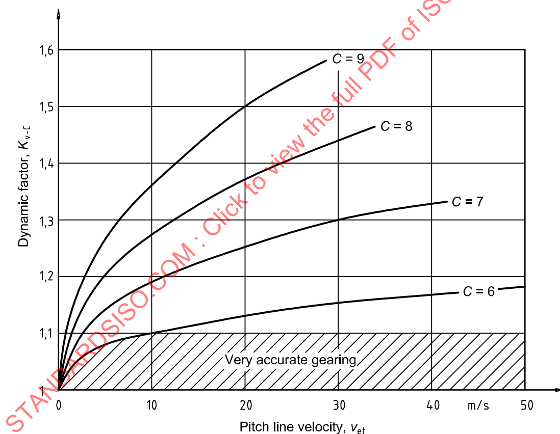
Figure 3 — Dynamic factors, K_{v-C}
