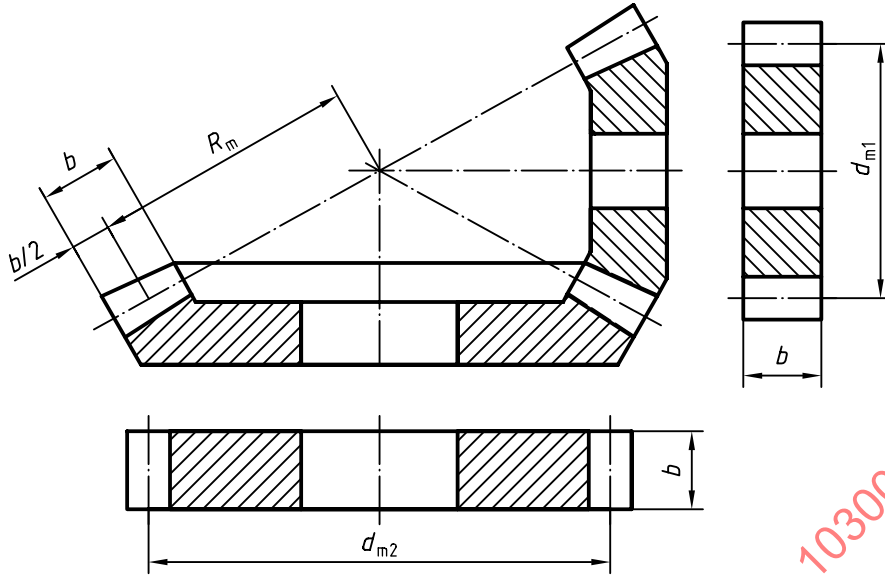
Figure 1 — Approximately dynamically equivalent cylindrical gears for the determination of the dynamic factor
