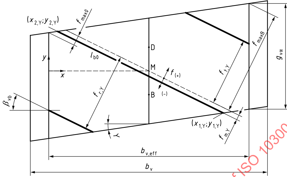
Figure A.7 — General definition of length of contact lines for local geometry data
