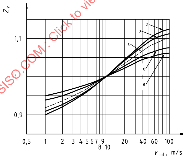
Figure 3 — Lubricant factor, Z_L
