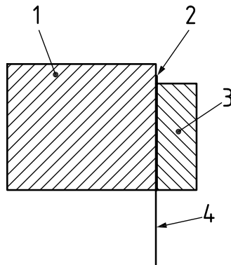
Figure 1 — Test plenum (full size)
