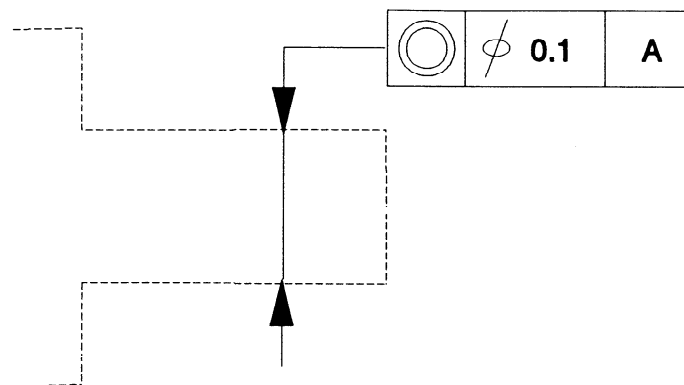
Figure 7 - Dimension curve directed callout
