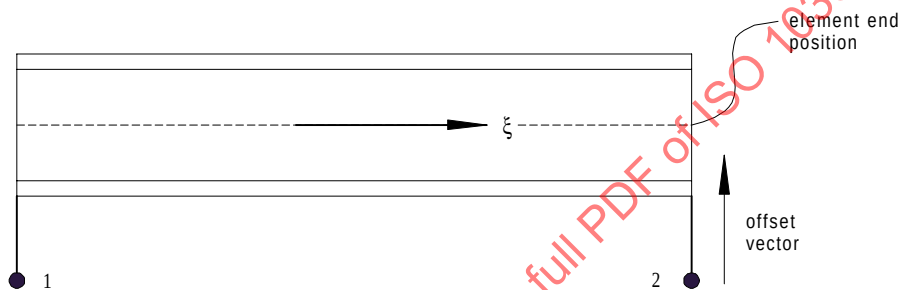
Figure 57 – Curve element end offsets
