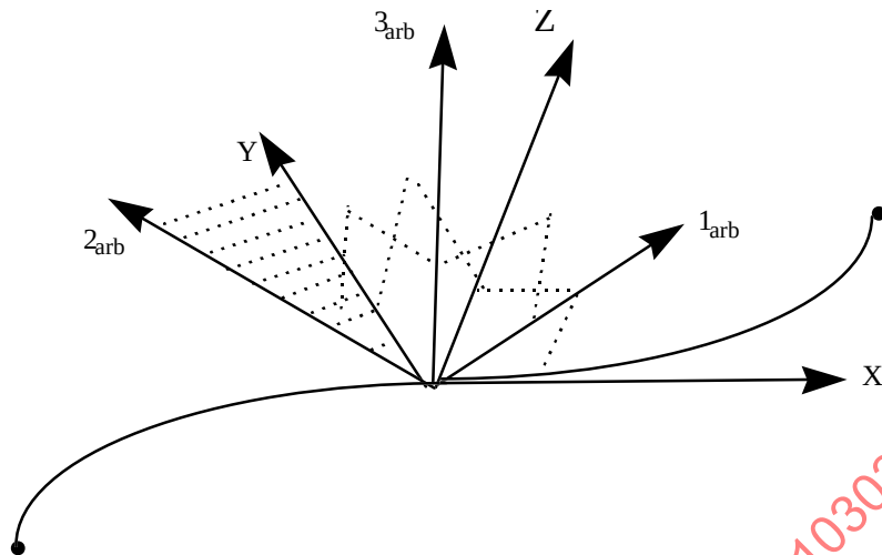
Figure 47 – Aligned curve 3D element coordinate system derivation
