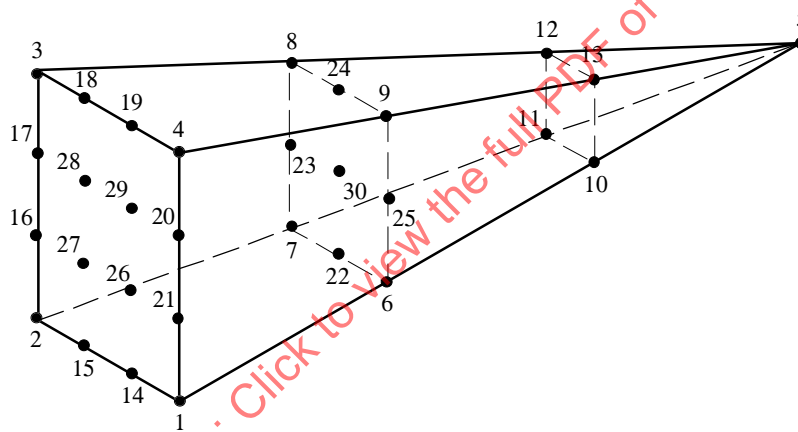
Figure 38 – Volume 3D elements - pyramid - cubic
