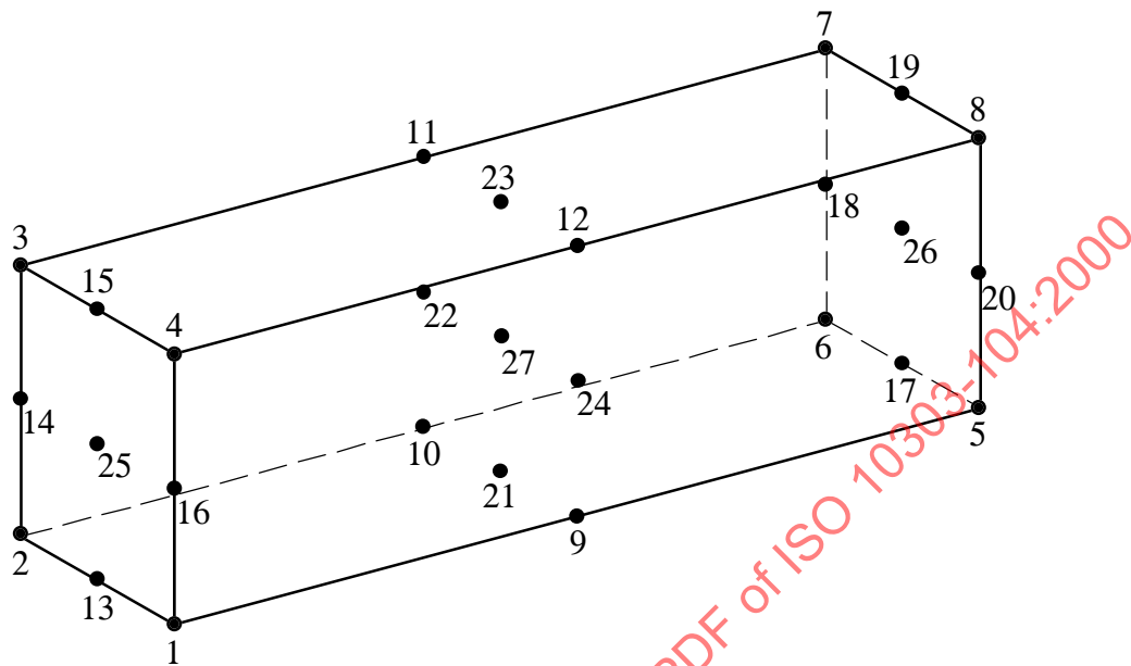
Figure 25 – Volume 3D elements - hexahedron - quadratic
