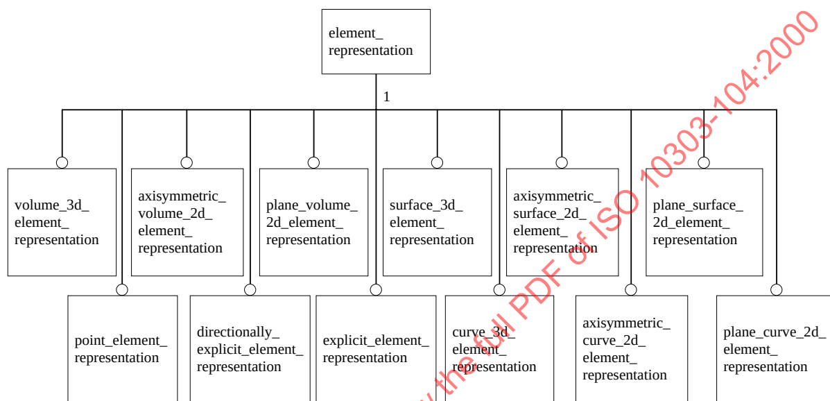
Figure 7 –Element subtyping
