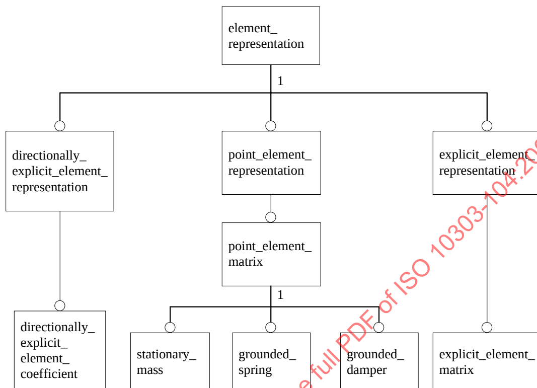
Figure 9 – Point, directionally explicit and explicit elements EXPRESS-G partial model
