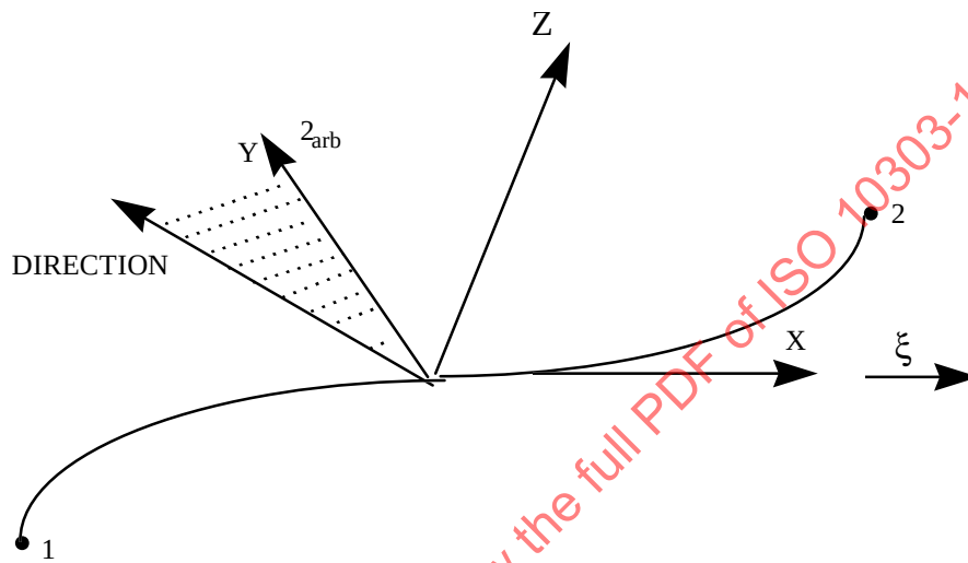
Figure 48 – Parametric curve 3D element coordinate system derivation
