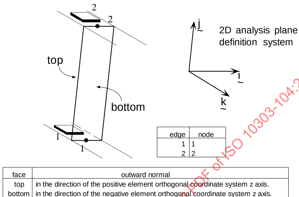
Figure 13 – Surface 2D elements - faces and edges
