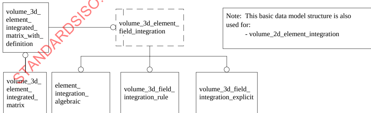
Figure 52 – Volume element integration EXPRESS-G partial model
