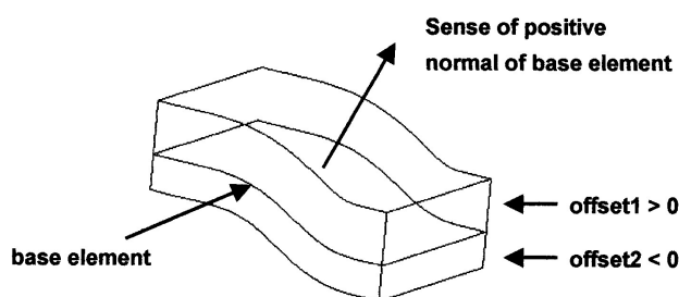
Figure 25 – Thickened face solid
