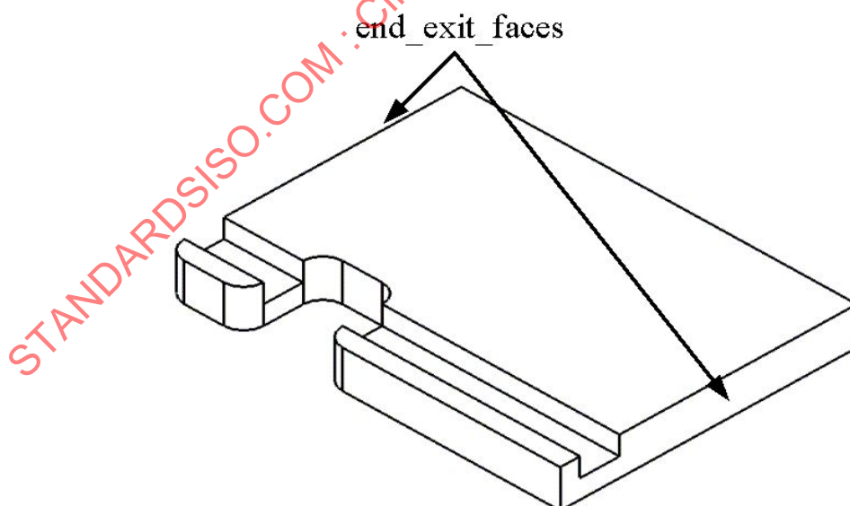
Figure 18 – Straight slot with multiple entries and exits from part material
