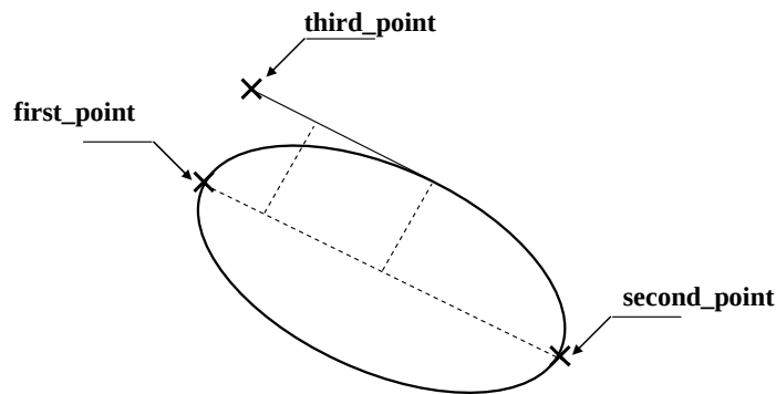
Figure 16 — create_ellipse_3_points
