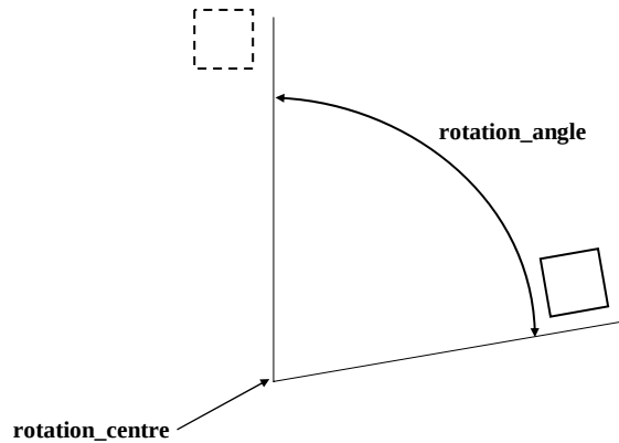
Figure 24 — sketch_transform_rotate
