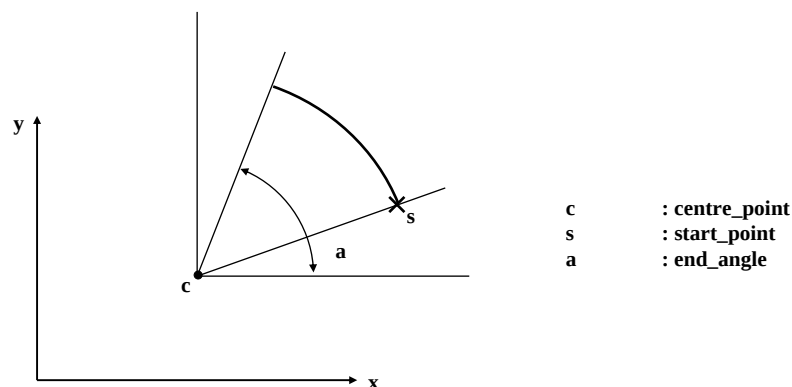
Figure 9 — create_circular_arc_start_centre_angle
