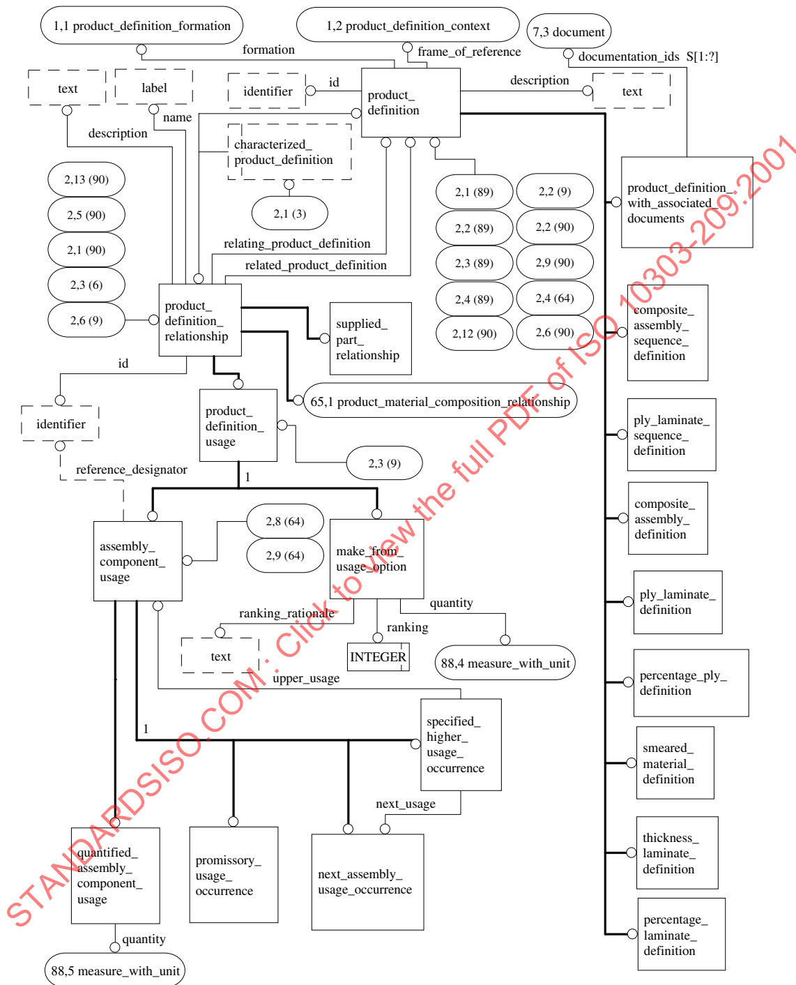
Figure H.2 - AIM EXPRESS-G diagram 2 of 94
